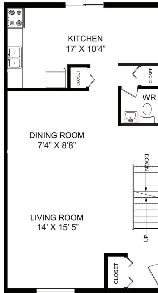
MAIN FLOOR
