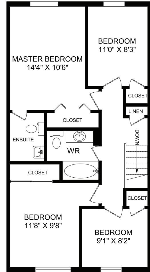
SECOND FLOOR
