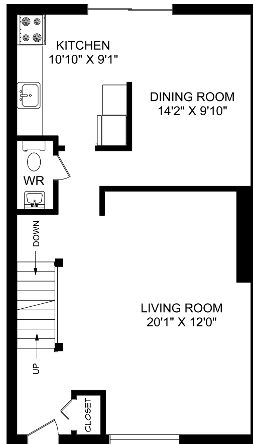
MAIN FLOOR
