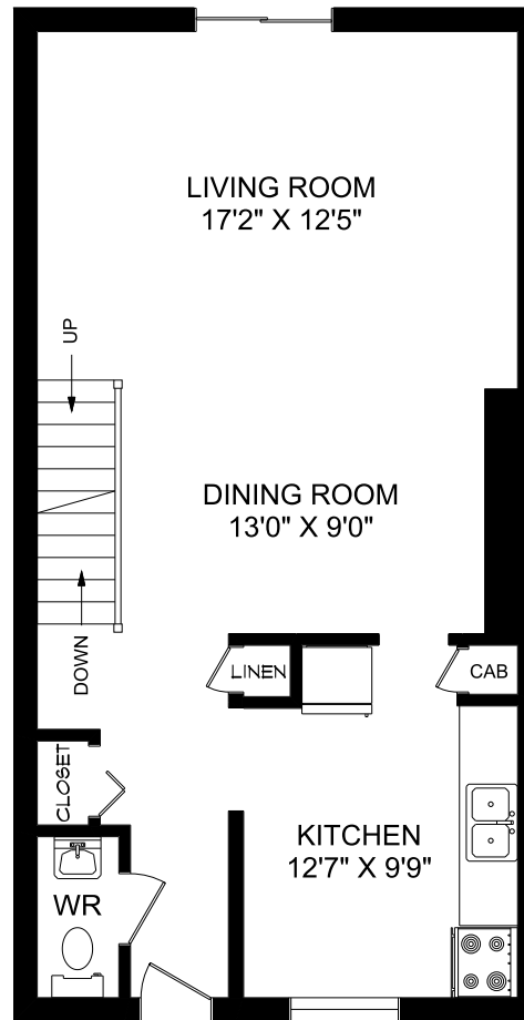
MAIN FLOOR
