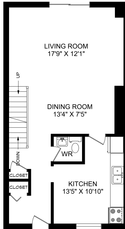
MAIN FLOOR
