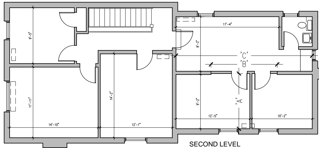
SECOND LEVEL 1,179 SQ. FT.
