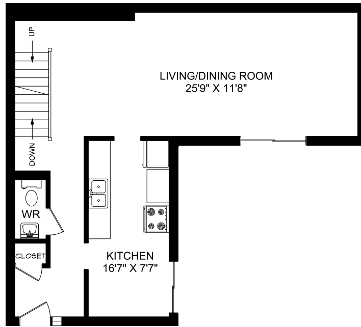
MAIN FLOOR
